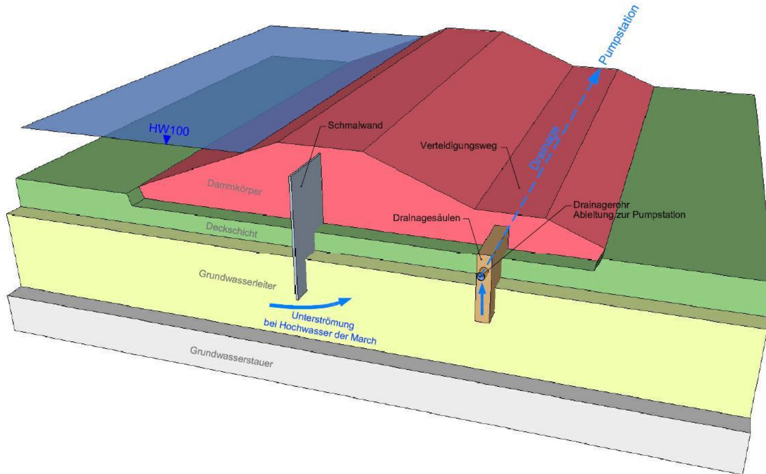
Schematic diagram of Flood Protection Morava river, Flood Protection Danube river identical
